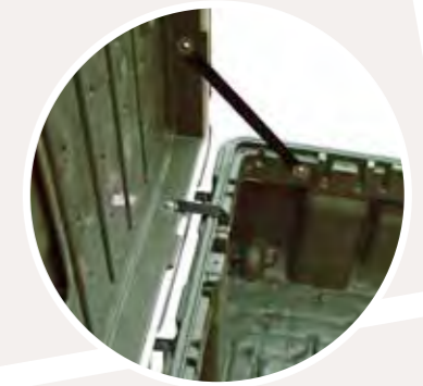
Webbing lid stays
